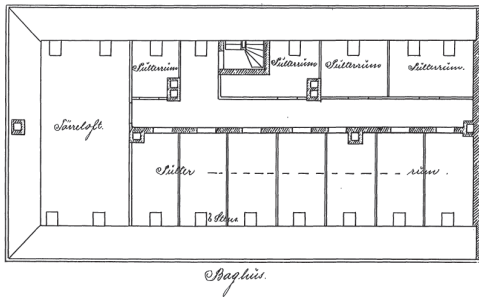
Laftplan
